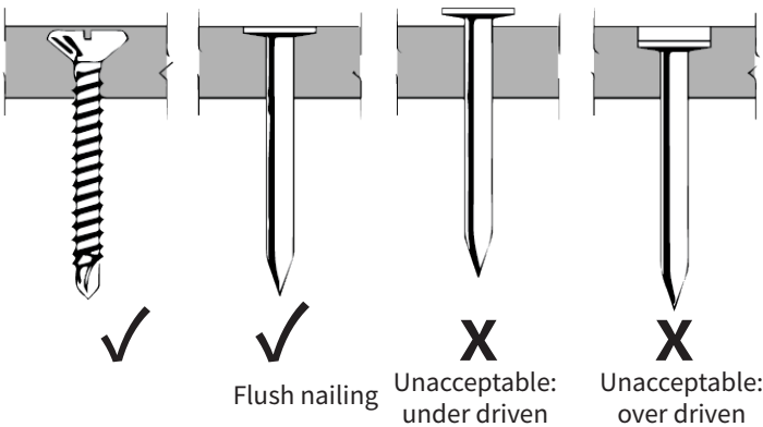
Figure 8 Fastener depth
